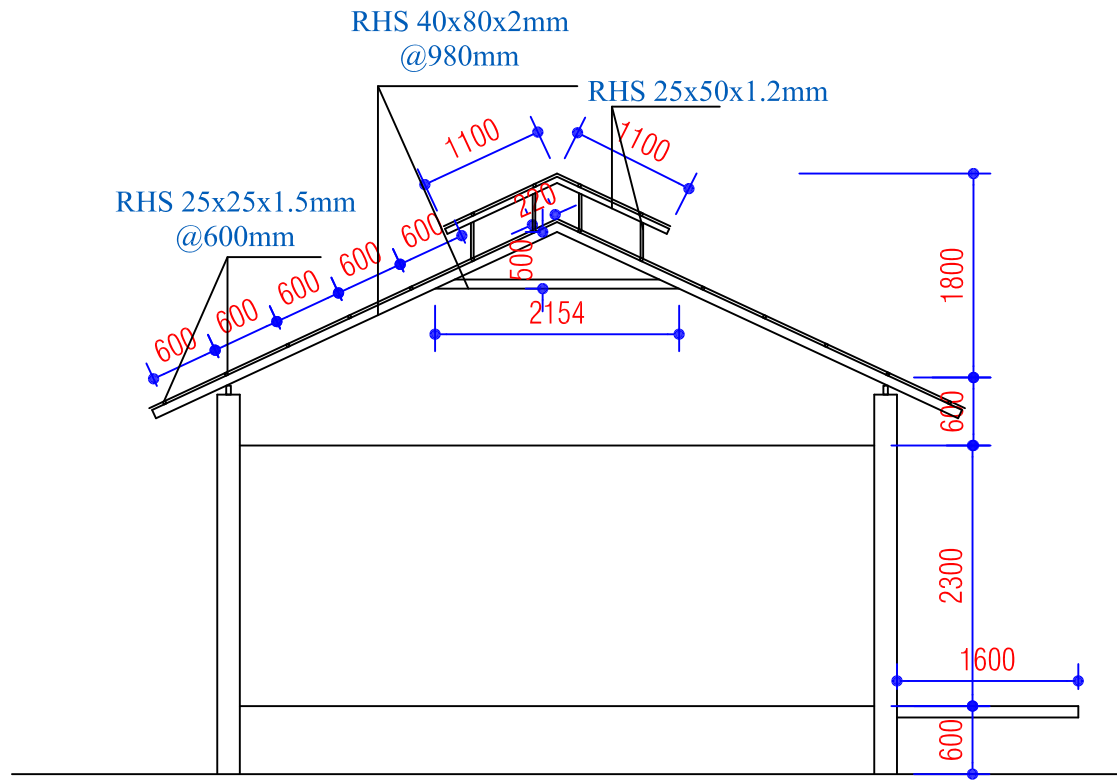
Frame Detail
